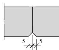
CEWOOD acoustic panel edge profile P5
