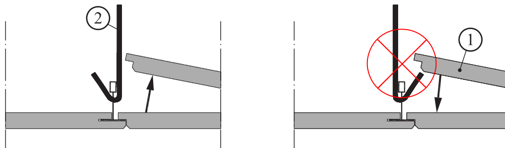
Fig. 7.5. Orientation of quick suspension mounting.
