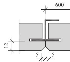
CEWOOD acoustic panel edge profile P5H
