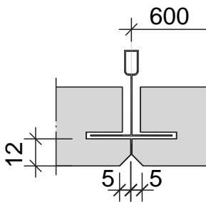
Fig. 4.1. CEWOOD acoustic panel edge profile P5H.
