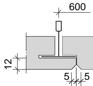
Fig. 4.2. CEWOOD acoustic panel edge profile P5S.
